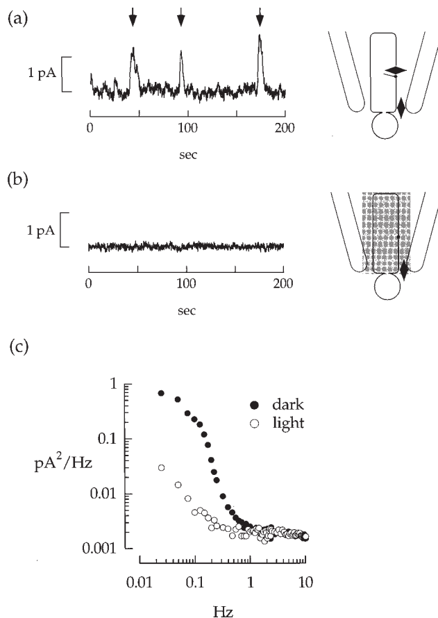
FIG. 6. Dark noise. (a) Fluctuations in the current collected by the suction electrode in darkness. These fluctuations come from two sources (schematic on right): cellular noise due to fluctuations in the current flowing into and out of the outer segment, and instrumental noise, including fluctuations in the current flowing across the seal of the outer segment into the suction electrode. The arrows mark three discrete photonlike noise events (see text). (b) Instrumental noise from the same cell as in (a). All the channels in the outer segment have been closed by exposing the cell to a bright light, leaving only instrumental noise. (c) Power spectra of the current fluctuations measured in (a) and (b).
